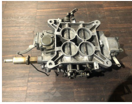
Holley Vergaser (Holley carburetor)
